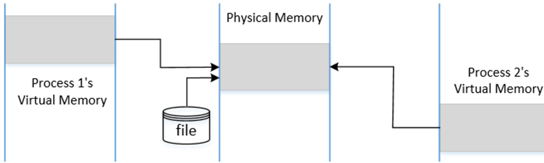
(a) MAP_SHARED
