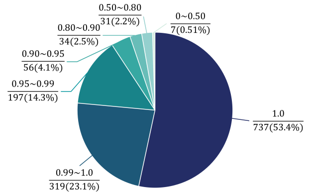
Figure 5: Cosine similarity of WEB mapping
