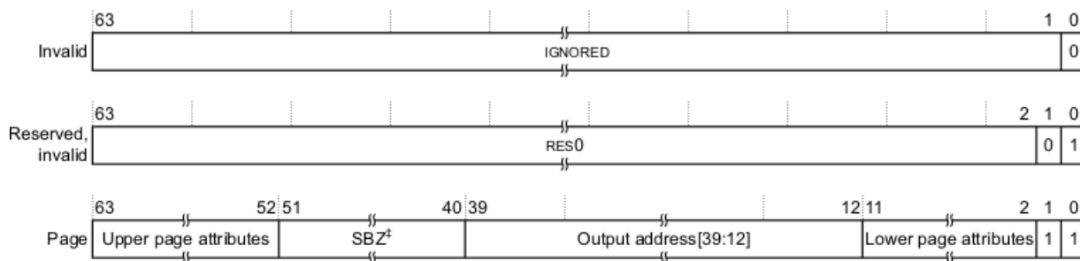
Figure 12: Structure of the level 3 table entry (descriptor)
