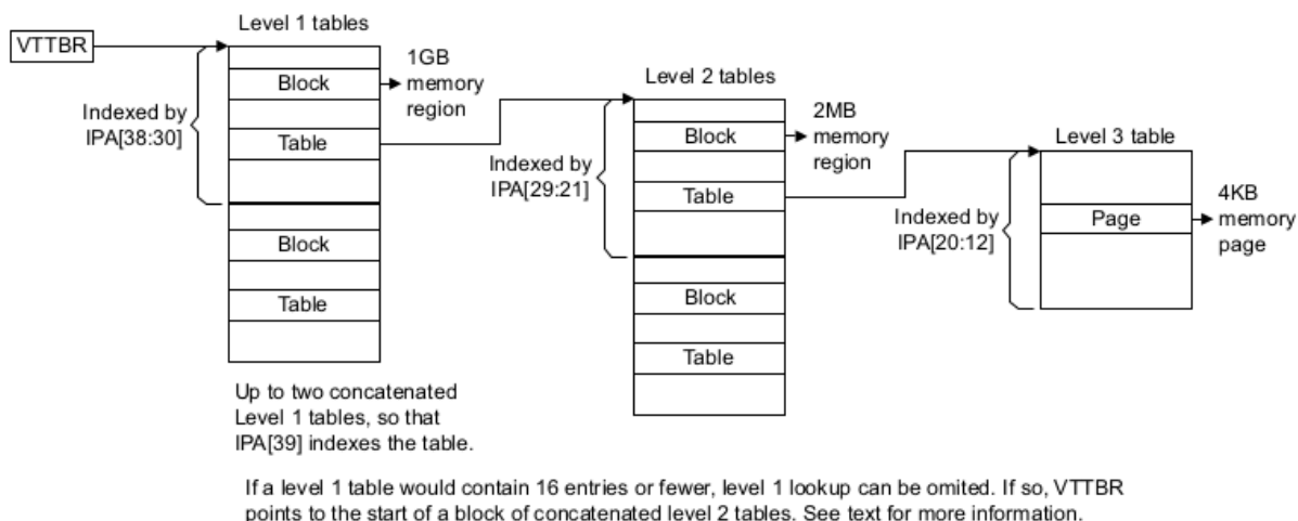
Figure 10: Stage-2 translation overview
