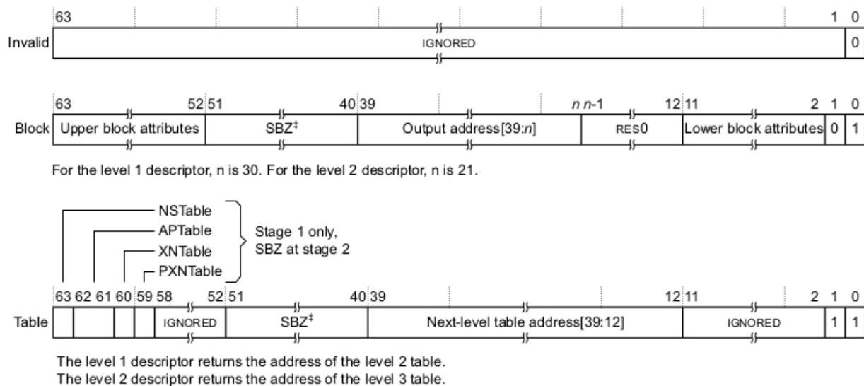
Figure 11: Structure of the level 1 & 2 table entry (descriptor)
